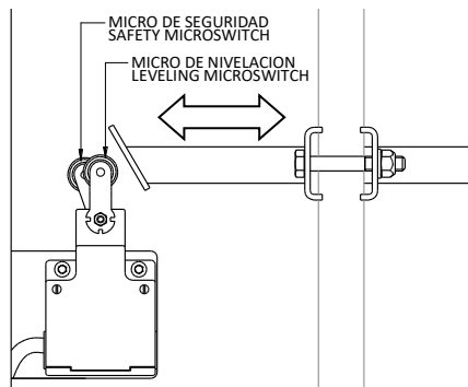
REGULACION LEVA
