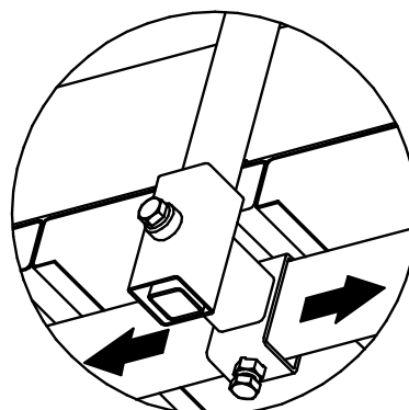
PORTAPOSTE LATERAL 086.4810
