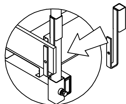
PORTARODAPIE LATERAL 086.405
