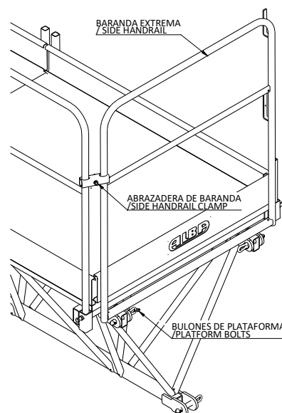
BARANDA EXTREMA
